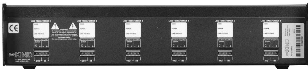
In / Out connectors rear panel
